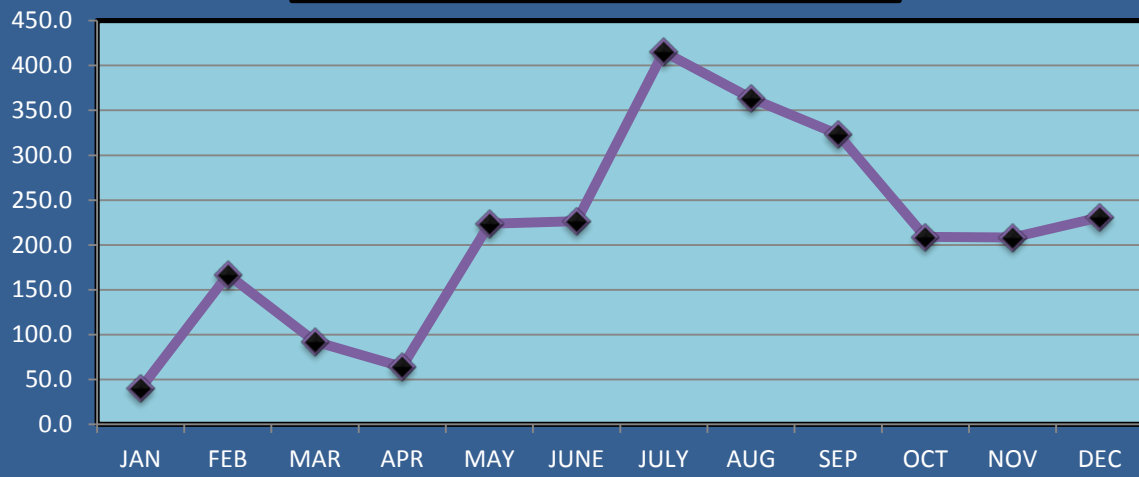
Rainfall 2001 (mm)
