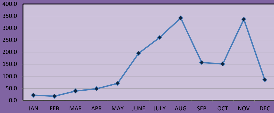
Rainfall 2003 (mm)
